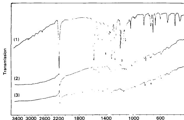
Fig. 1. IR spectra (KBr pellets) at room temperature. (1) Pure M_2P -TCNQ; (2) P_{0.4}(M_2P)_{0.6}TCNQ ; (3) NMP-TCNQ.
